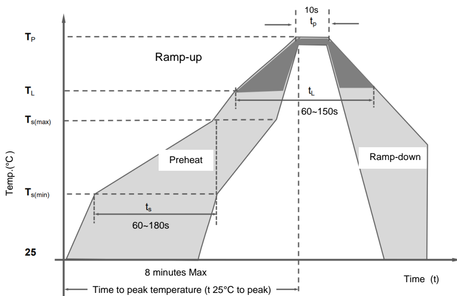
Figure 9. Reflow Soldering
