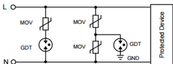
Figure 7. AC Power Input Protection Circuit
