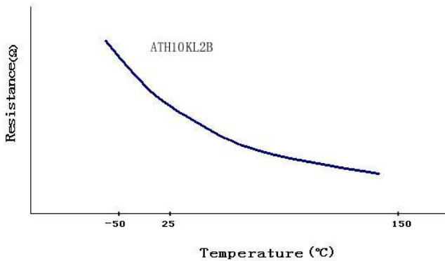
Figure 4. Resistance vs. Temperature for ATH10KL2B
