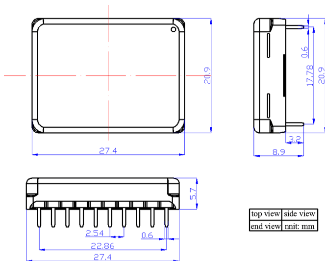
Figure 12. Dimensions of the DIP Package Driver
