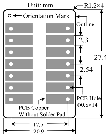
Figure 14. Top View of the Top Side PCB Foot-print
