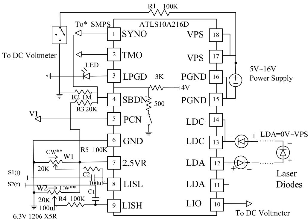
Figure 7. Application With Modulation Circuit
