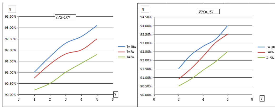
Figure 6. Efficiency of Laser Driver
