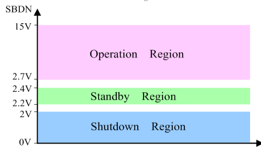
Figure 4. Input Control
