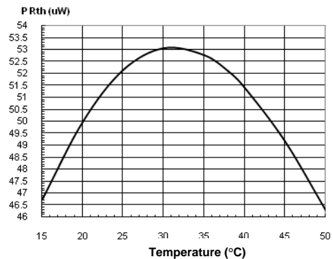
Figure 11. PRth vs. Temperature
