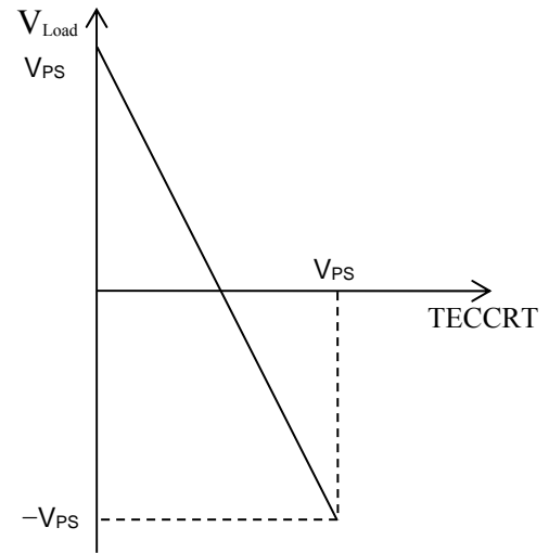
Figure 13. V_{Load} vs. TECCRT
