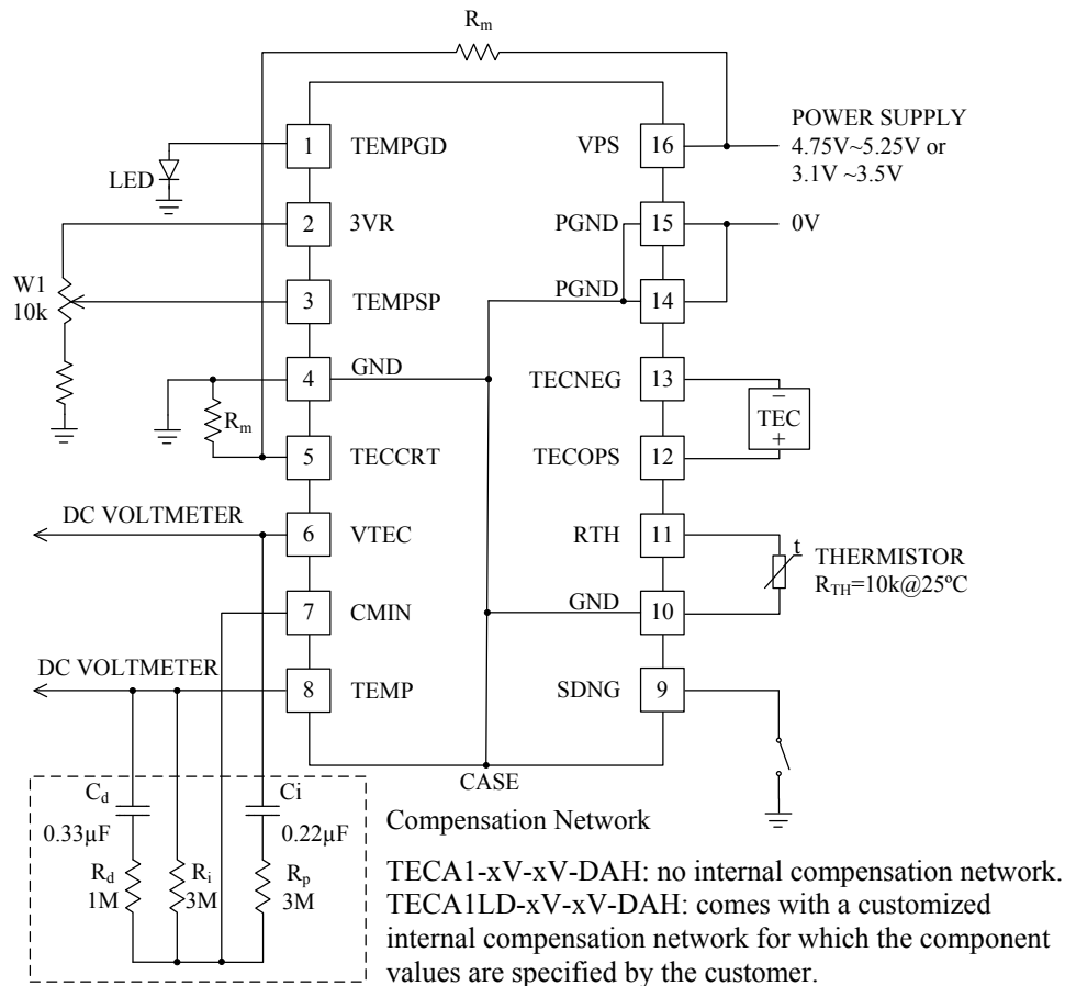
Figure 5. Stand-Alone Application Circuit
