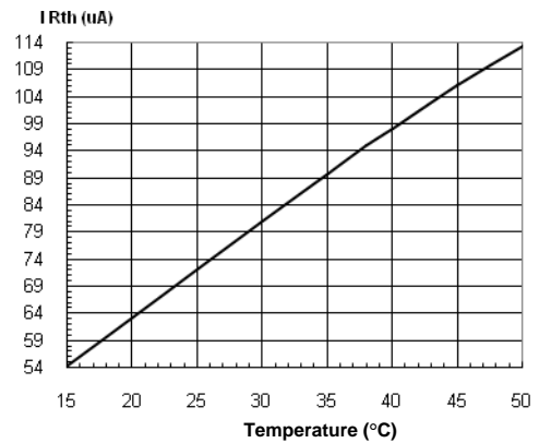
Figure 10. IRth vs. Temperature
