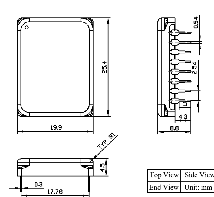
Figure 19. Dimensions of the DIP package controller of TECA1-xV-xV-DAH
