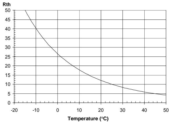
Figure 8. Rth vs. Temperature
