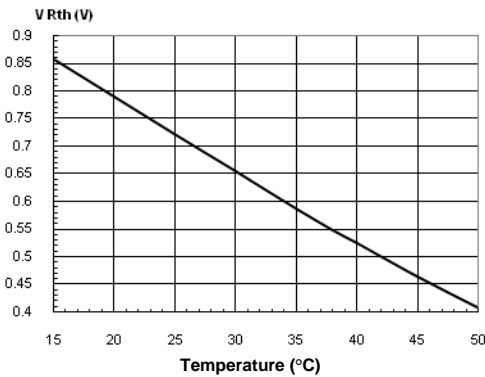
Figure 9. VRth vs. Temperature
