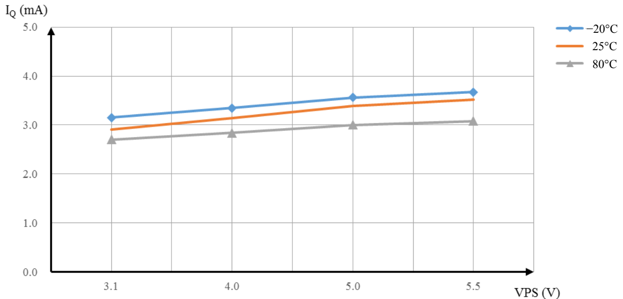
Figure 14. V_{PS} and Temperature vs. I_Q
