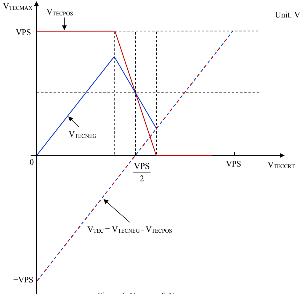
Figure 6. V_{TEC_{MAX}} & V_{TEC_{CRT}}
