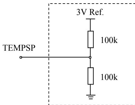
Figure 17. Internal Equivalent Circuit on TEMPSP Pin
