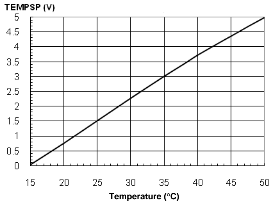
Figure 12. TEMPSP vs. Temperature
